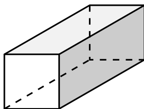
rectangular prism
