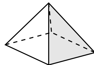
square pyramid
