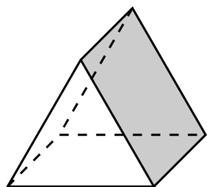
triangular prism
