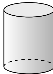
cylinder
