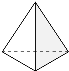
tetrahedron
