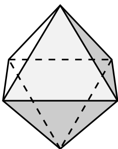
octahedron
